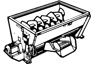
Stationary weigher-mixer
