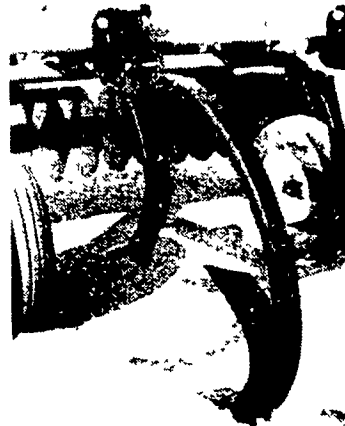
Rigid shanks are recommended for use in soils free of rocks and stumps. Shear pin protection is standard equipment. Shanks contact the soil at a reduced angle, requiring less HP and fuel.
