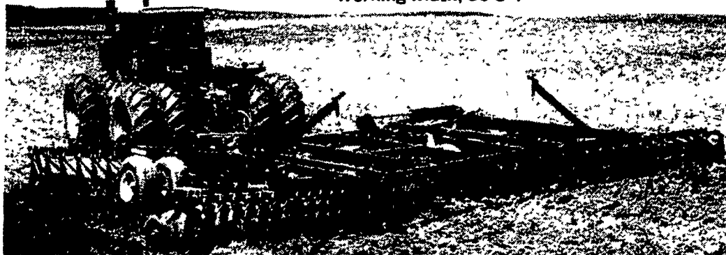
Model 2455 Heavy-Duty "Flex-Wing" Tandem Disc Harrow. Working width, 35'8".
