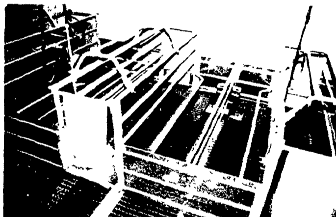
5 Farrow Rooms With 12 Crates Each, Woven Wire Fencing, European-Style Crates
