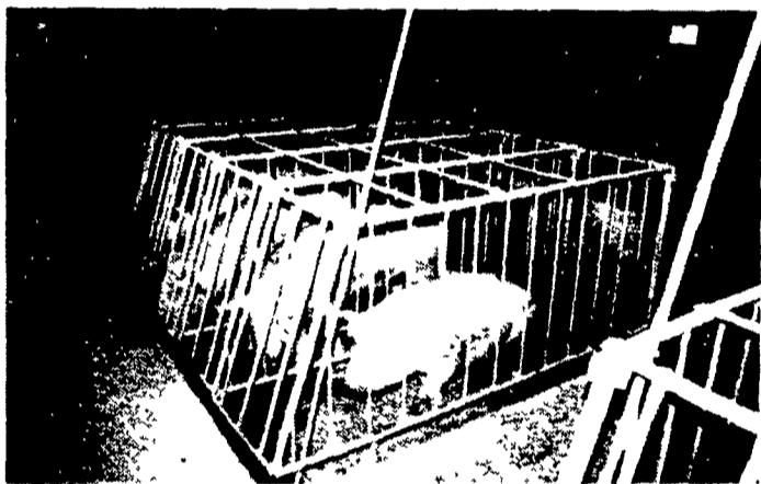
Hot Dipped Galvanized Gestation Stalls, Concrete Slats And Trough
