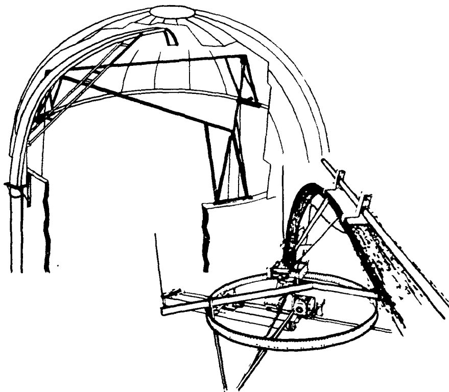
VOLUMATIC III silage distributor/unloader
