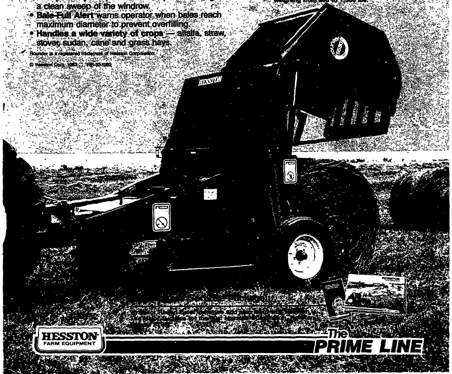
Three other open-throat Hesston round balers produce 4x8', 5x5', or 5x6' high-density bales weighing from 800 to 1,500 lbs.
