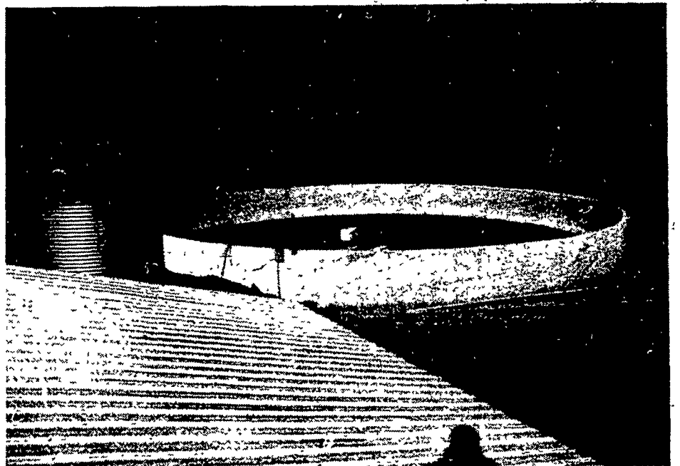
Concrete Tank With Aerator For Recycling Waste Water To Flush Manure From The Barn
