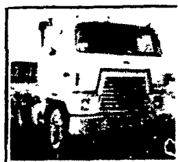
1978 IHC CDF4070; T/A/D/S; 142" WB; 8V-71TT Detroit 305 HP EATON DS380 R.A., RT9509, 9 Speed, A/C, P/S.
