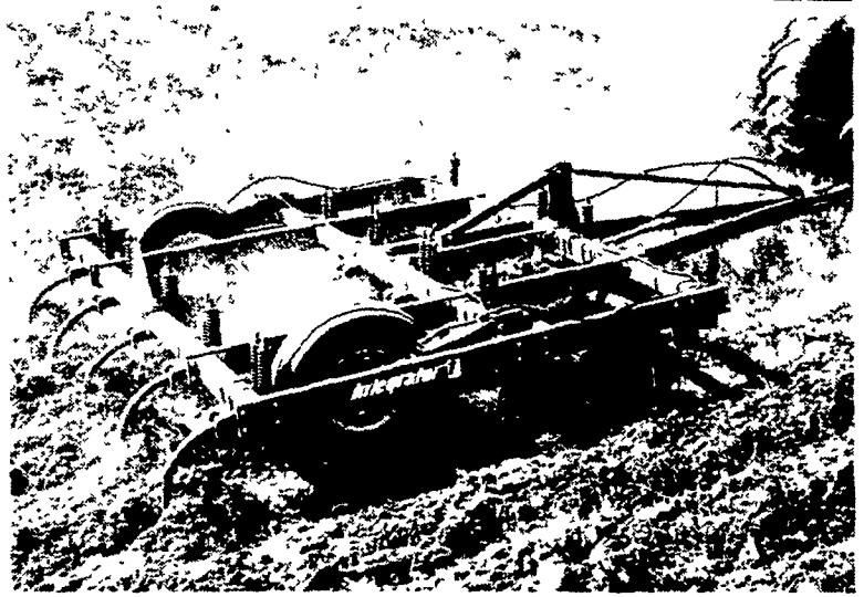
The Kewanee Integrator 1 coulters chisel, primarily a fall tillage tool and the first of a series of three Integrator implements Chromalloy Farm Equipment Division will introduce, is equipped with 4-inch wide helical blade till points and 20-inch by 5 mm coulters.
