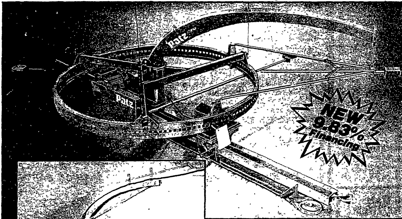
Patz double-hook gathering chain features knife-sharp cutters and claws for full-flow feeding.
