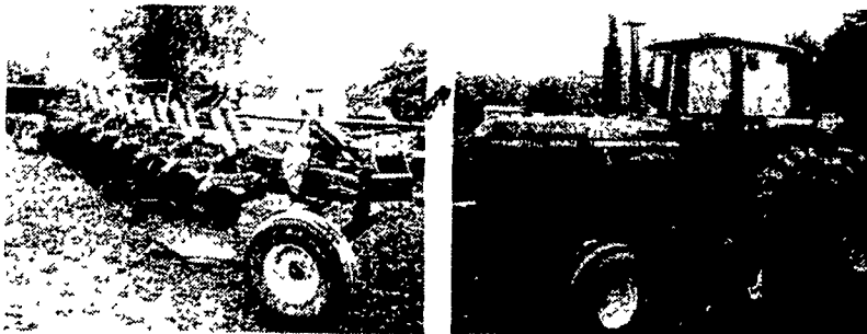
Used JD 2500 7-Bot., Spring Trip, on Land, Fits our JD 4640 Tractor
