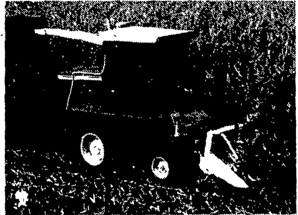
Hesston/Field Queen Self-Propelleds feature a power-efficient, 6-knife cutting cylinder and giant 139 sq. in. throat opening for big tonnage forage harvesting. Exclusive Hesston Flo-Vanes on the 7650 and 7600 reduce bunching and increase capacity. The big Command Post Cab offers unmatched comfort and convenience. Add the industry's widest selection of SP headers, and you have the prime cut!
