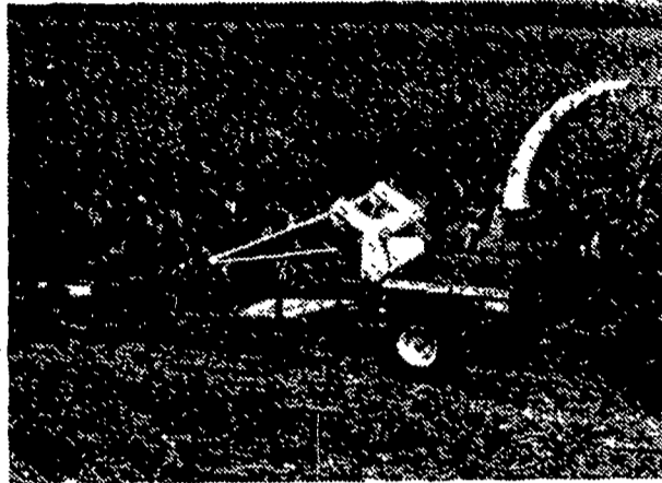
Hesston 7100 Series Pull-Type Forage Harvesters feature a precision-built, 6-knife cutting cylinder. It doesn't "chop" crop...it "slices" with scissor-action efficiency for clean cutting, top capacity and fuel efficiency! Straight-through crop flow puts more power into cutting the crop, and exclusive Flo-Vanes add even greater capacity!
