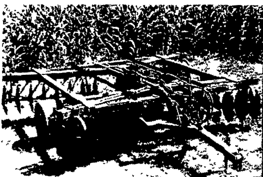
6722 - King Model #AOWL disk, Disc: width 12', Tandem, Blades spacing: front 9", rear 9", size: front 22", rear 22"
