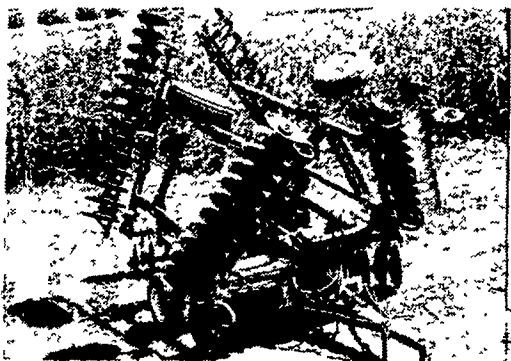
6021 - Krause 1928 Rockflex Disk, 25' Flexwing Disk, Blades spacing: front 8", rear 8", size front 22", rear 20"
