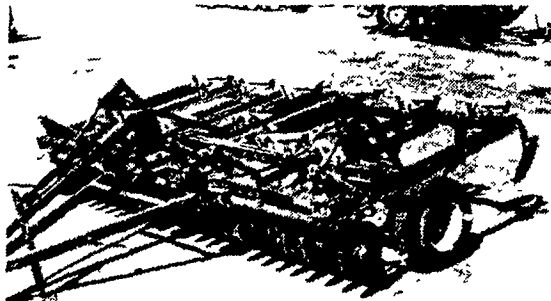
6493 - Glencoe SSP 22 Soil saver, 11 shank, s/n 119300, 15' disc, Blades spacing: front 7 1/2"
