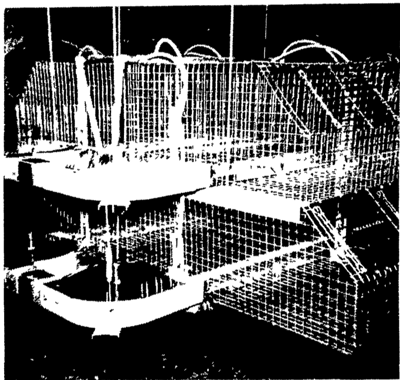
Pullet Grow Cage System
