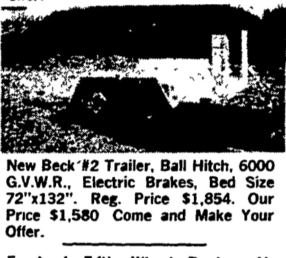
New Beck #2 Trailer, Ball Hitch, 6000 G.V.W.R., Electric Brakes, Bed Size 72"x132". Reg. Price $1,854. Our Price $1,580 Come and Make Your Offer.
