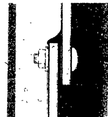
Cross-section view shows how sheets are joined together. Sealer flows between sheets and around plastic-capped bolt to assure a tight joint.
