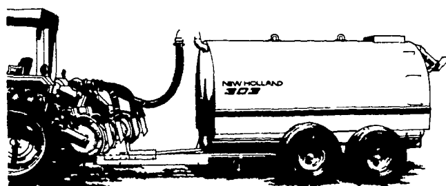
TANDEM AXLE LIQUID TYPE 2,222 OR 3,264 GALLON CAPACITIES 3 POINT HITCH INJECTOR OR BROADCAST
