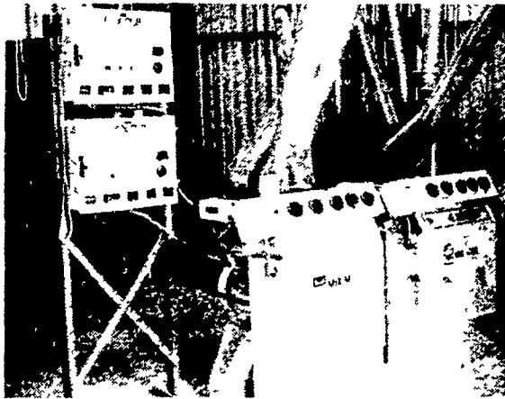
THE FAMOUS MIX MILL SYSTEM
