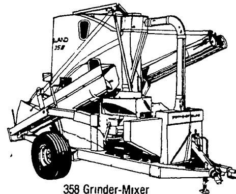
358 Grinder-Mixer 125 Bu. Tank with 21" Mill
