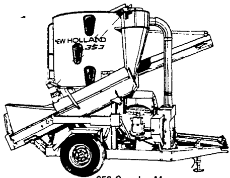
353 Grinder-Mixer 80 Bu. Tank with 16" Mill
