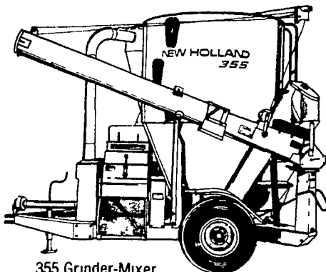
355 Grinder-Mixer 100 Bu. Tank with 21" Mill
