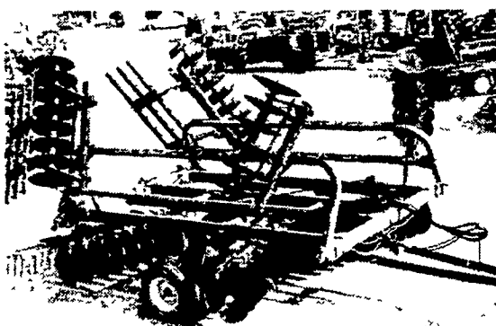
Deere 230 Tandem 25' Cut, with Mulchers
