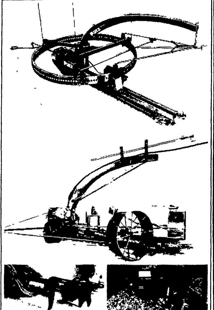
Patz double-hook gathering chain features cutters and claws
