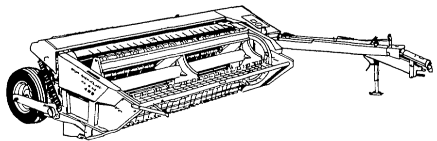
MODEL 489 MOWER-CONDITIONER
