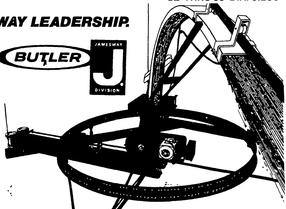
Collector ring features vertically mounted copper alloy rings and big spring-loaded brushes. You get uninterrupted power
