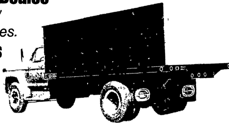
Steel body shown with optional 12" tip tops, which are available on 28", 40" and 52" steel sides in all lengths.
