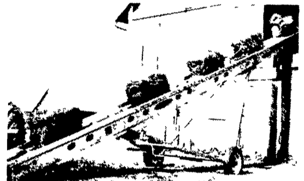
With 19" Slat Spacing, Heavy Duty No. 62 Chains & Shovel Hopper, Ideal For Corn Handling, Set Up, Prices F O B Dealers Lot
