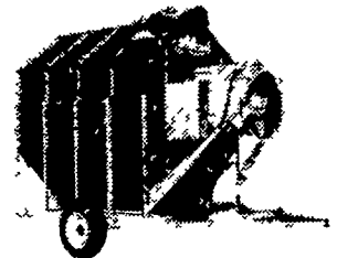
AB Model—8B "Temper Dries" to 210 bu per hr
