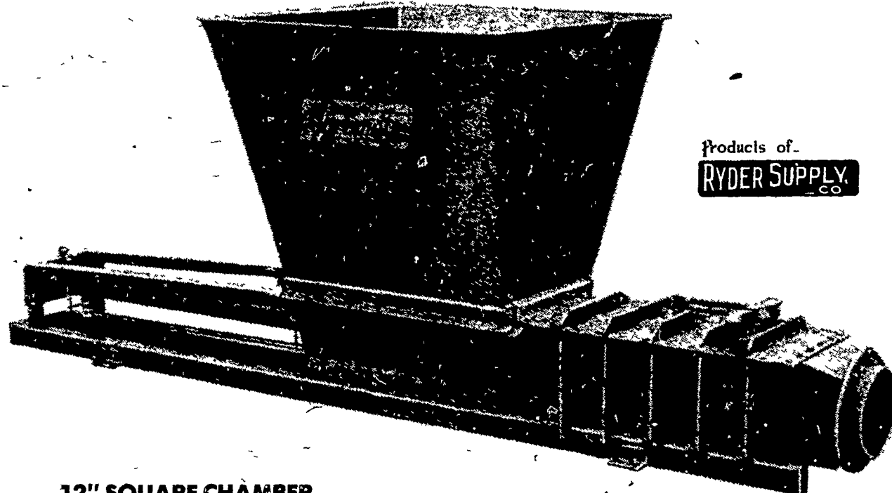
HOPPER is 8 gauge steel and 42" square. Optional longer hopper is standard. The base of the hopper assures proper plunger alignment as it enters the chamber.
