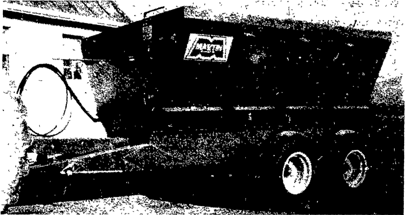
All Martin spreaders are equipped with floating beam tandem axles. Choose from nine standard models, 1,575 to 4,500 gallons, or custom built to your order. Design top opening to your size requirements, with hydraulic lid optional.
