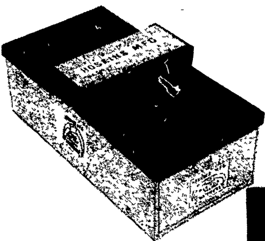
H9-14D 5 Gal. S.S. Tank. Serves: 100 Head. Length: 28". Height: 9". Width: 14". Weight: 55 lbs. 250 Watt Heat Unit.
