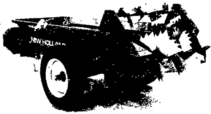
MODEL 213 , shown with upper beater, does a fine job of topdressing. Capacity 139 cu. ft.
