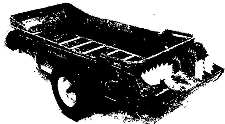
MODEL 519 , here equipped with hydraulic endgate, will spread either wet or dry manure without adjustment. Capacity 216 cu. ft.
