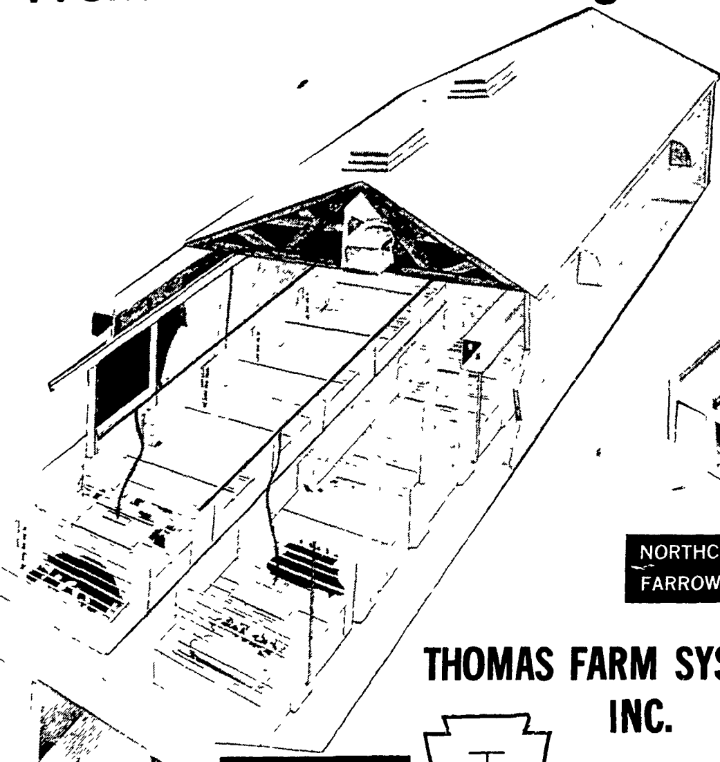
NORTHCO CENTER PIT FARROWING SYSTEM
