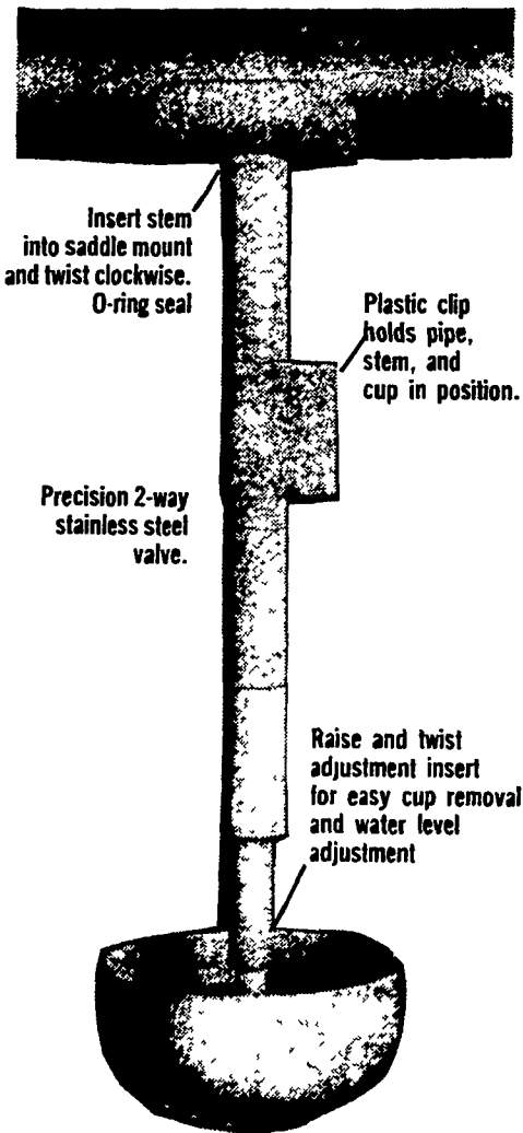
Pipe with saddle mounts spaced to fit any type cage arrangement.
