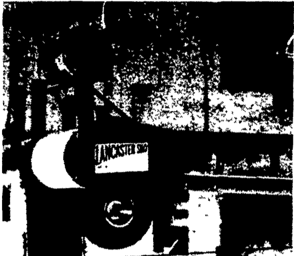
Belt Feeder mounts overhead to allow clear feeding on bunk trough. Motor mount is adjustable. Rubber tire assures proper tension for belt travel.
