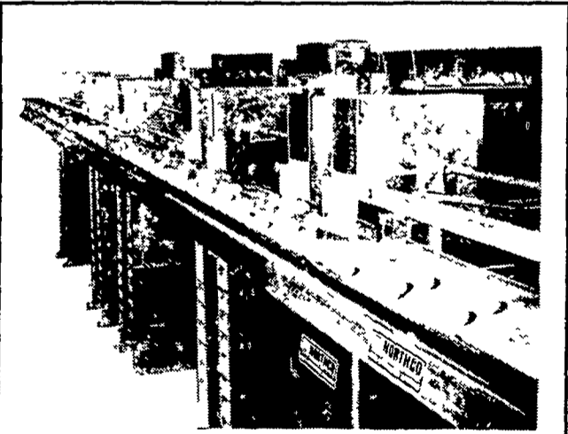
Northco egg gatherer Designed to be versatile, efficient, very gentle. Reduces checks and cracks 16" cross conveyor belt available.
