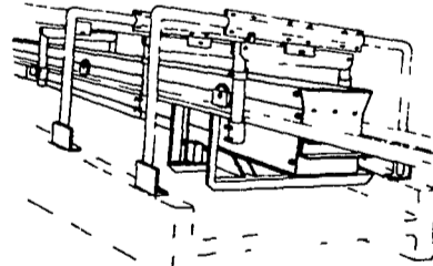
TRAVEL FEEDER
