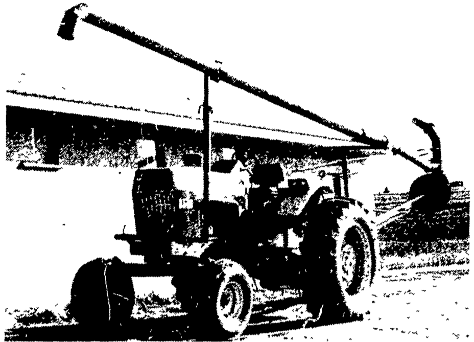
3 PT. HITCH LAGOON PUMP
