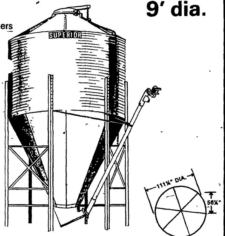
FOUNDATION DIAGRAM FOR 9' DIAMETER BIN
