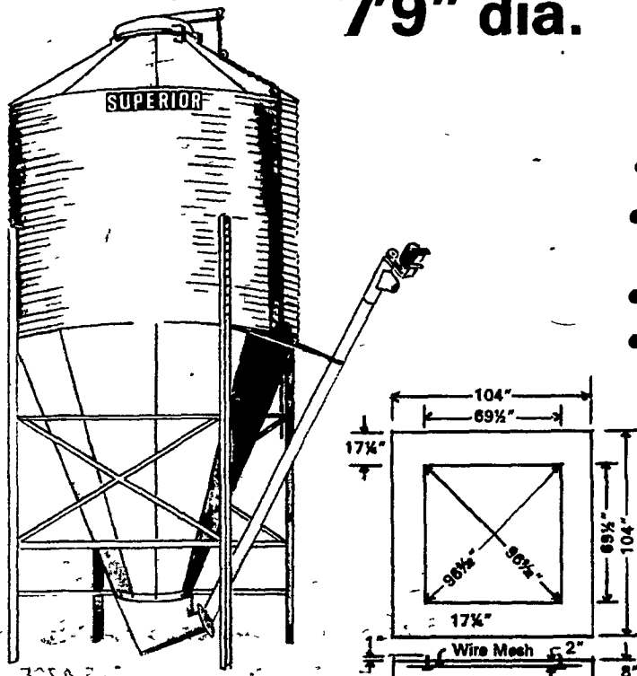
FOUNDATION DIAGRAM FOR 7'9" DIAMETER BIN
