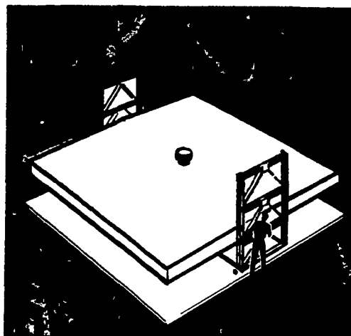
The entire roof structure and covering is completely assembled on the ground.
