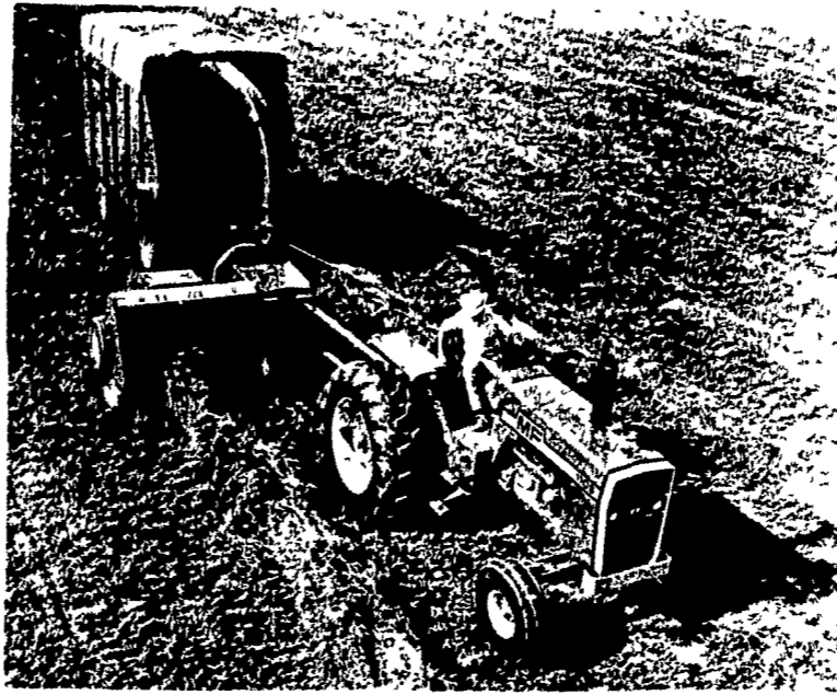
Massey Ferguson's new 260 forage harvester is designed for use with tractors from 90 to 175 hp. Twenty-six in., six knife cutter head and separate blower are standard. Harvester offers selection of four screen sizes, three harvesting attachments. Optional full remote control is available.
