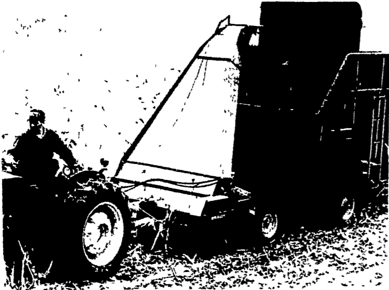
Brady model 722 Multi-Crop Chopper, designed for use in green-chopping hay, shredding corn stalks, weed mowing, chopping berry and grape vines, and a variety of other mowing and cutting jobs, features knives guaranteed against breakage. Model 722 offers full 72-in. cut and three discharge options.
