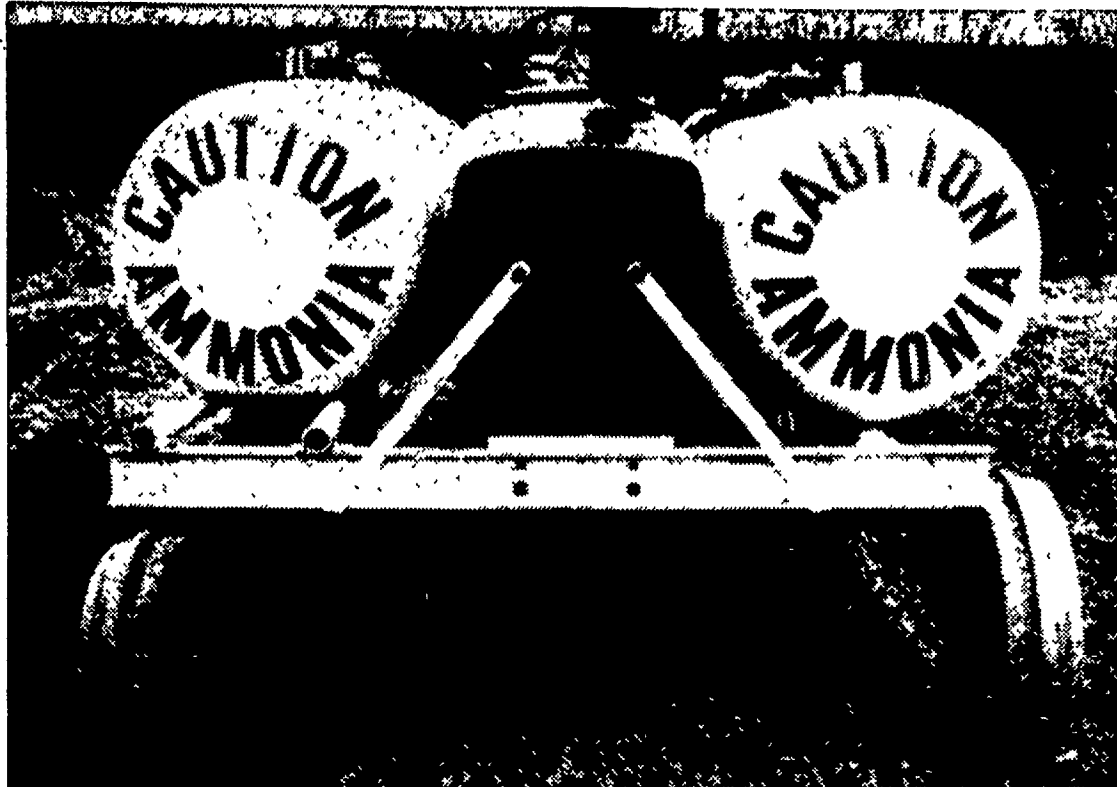
THE MOUNTING for this tractor was developed by engineers at Penn State University in cooperation with the U. S. Steel Co. It supports two applicator tanks of anhydrous ammonia, and was used at two locations in the county this week. Helping to make this material a low-cost fertilizer is the fact that every 100 pounds of anhydrous ammonia contains 82 pounds of nitrogen.
