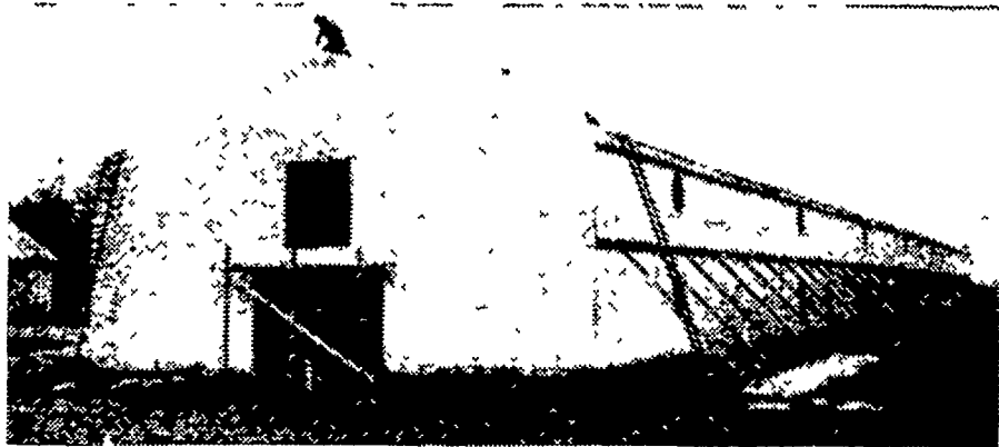
New controlled environment broiler house during construction stage — Farm of Richard Baker, Columbia, Pa.
