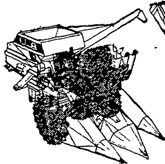
Uni-System combine with cornhead for top performance in "corn country" Greedy Superpicker Cornhead has specially designed snapping rolls, and double auger elevators to carry the ears off fast.
